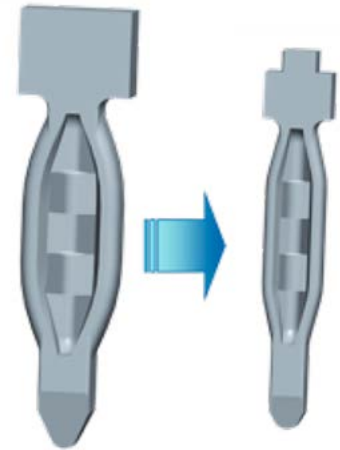
Picture 11 Standard Multispring and NanoMultispring pin.
