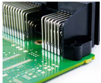
Picture 6 Pin Header 90° with press-fit pins inserted into the PCB.
