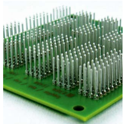
Picture 5 Stand-alone press-fit pins inserted into a PCB.
